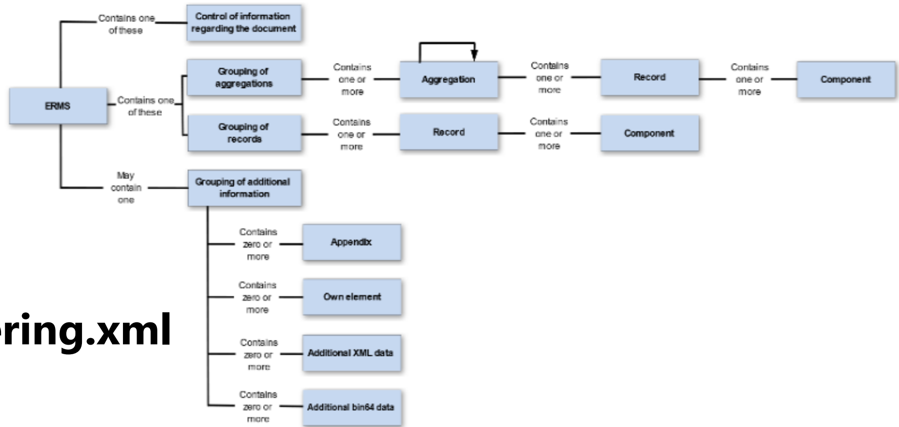
Figure 3: Components of the ERMS XML-format
